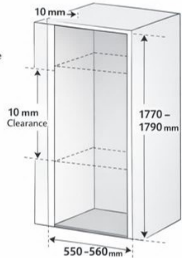
INSTALLATION SPACE
